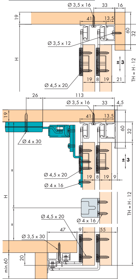
EKU-COMBINO 20/35
